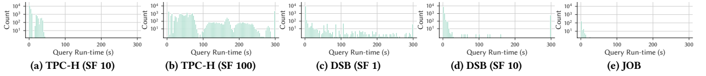
Figure 6: Query Run-time Distribution – Breakdown of elapsed time for each workload (without any acceleration).
