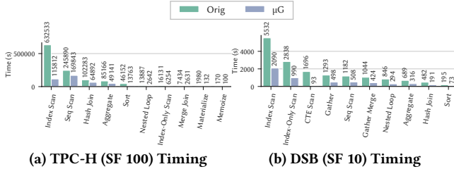
(a) TPC-H (SF 100) Timing
