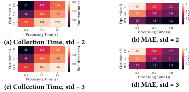
Figure 15: Batching Sensitivity – Collection time and MAE as we vary \mu G ’s hyperparameters on TPC-H (SF 10), 100 queries.
