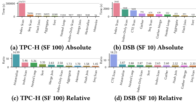
Figure 13: Speedup Analysis – Each operator’s speedup because of \mu G in Figure 12 (higher is better).
